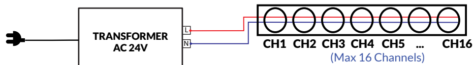
Connection Diagram Camaleon L RGB
